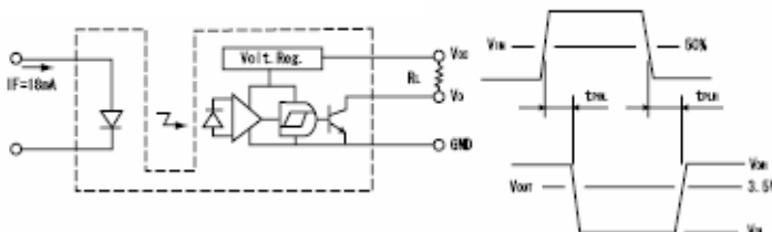
Measurement of propagation time
